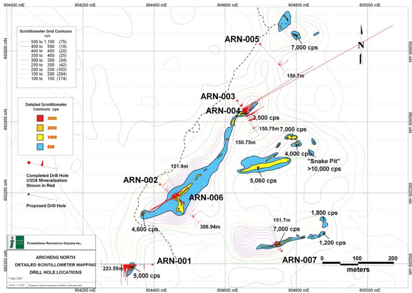
Figure 1: Aricheng North Detailed Scintillometer Mapping Drill Hole Locations
