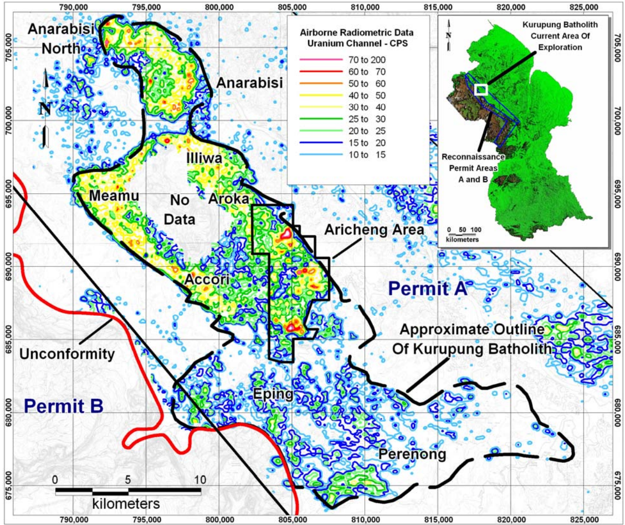
Figure 1: Kurupung Batholith Map
