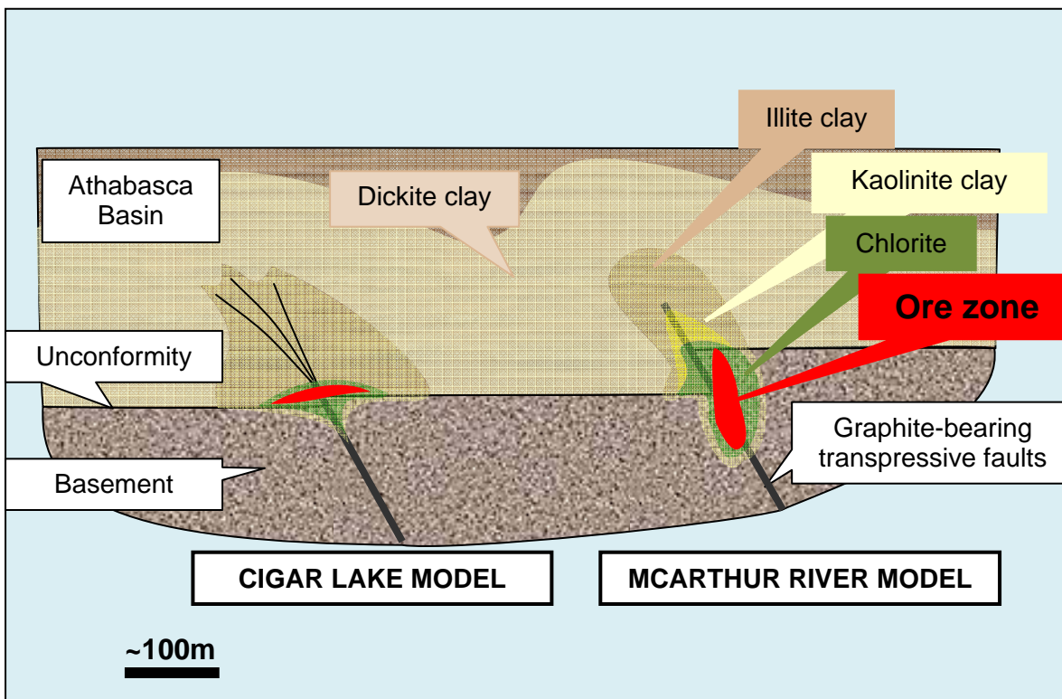
Figure 1: Diagram shows examples of unconformity-related alteration haloes associated with uranium deposits in the Cigar Lake and McArthur River mines in the Athabasca Basin. Specific clay minerals (eg. illite and chlorite) in alteration haloes can narrow exploration to within hundreds of metres of the ore body. U3O8 Corp. is adopting alteration mapping, as an indispensable and cost-effective tool, to focus its exploration for unconformity-type deposits in the Roraima Basin.
